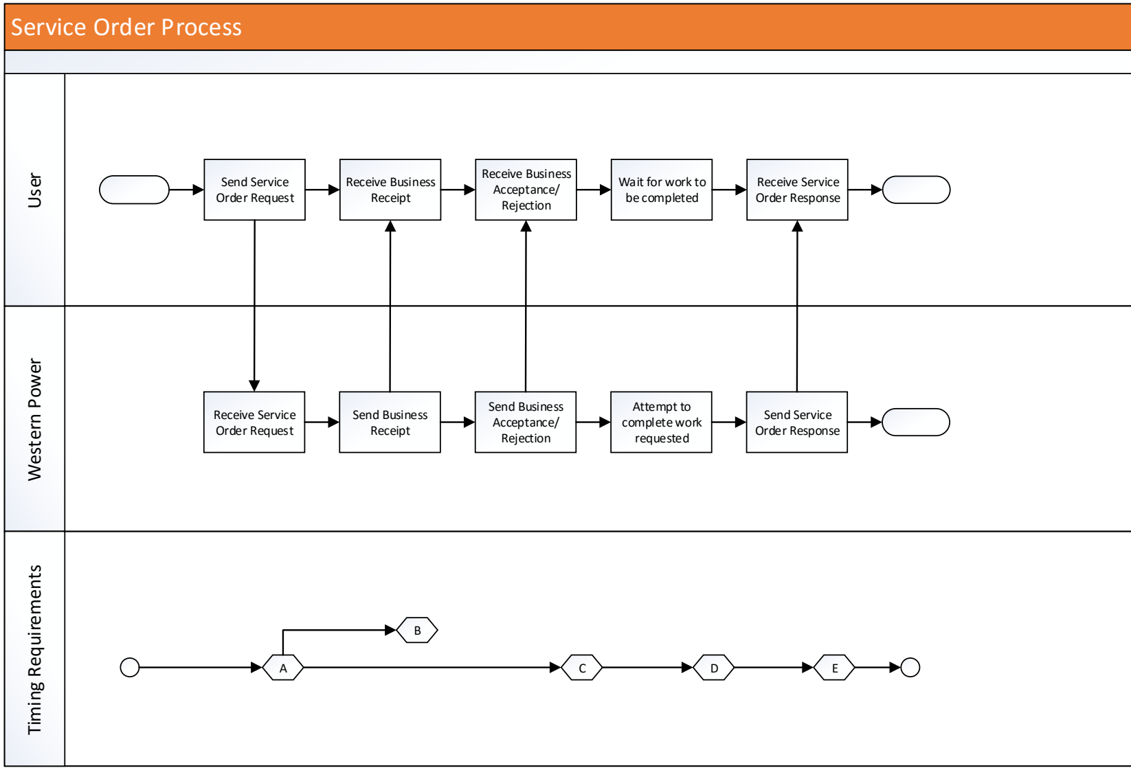
Figure 1: Timing Requirements
